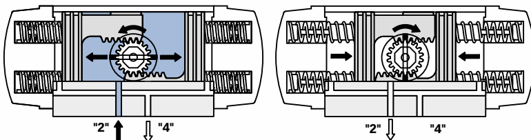
Fig. SC02: Top view and principle of a single acting actuator under spring pressure
