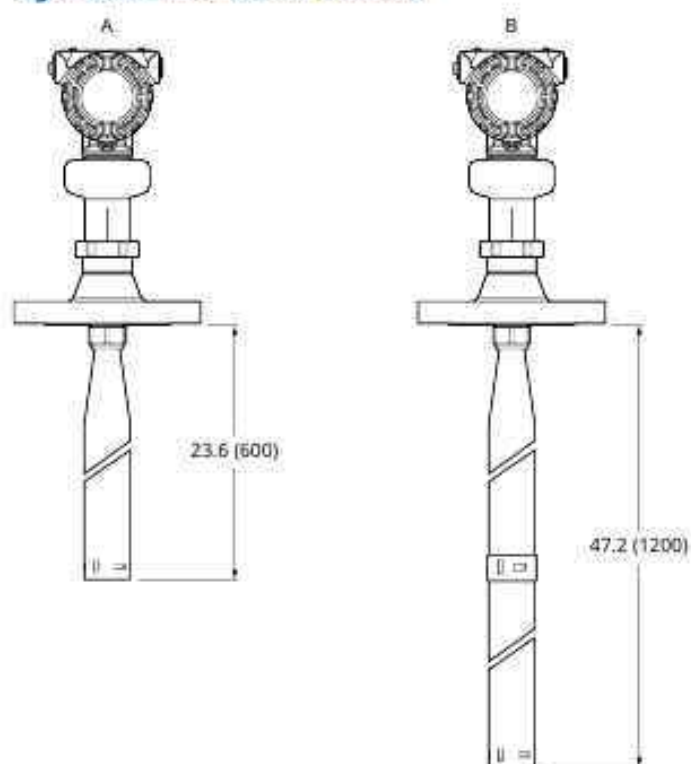
Figure 27: Extended Cone Antenna
