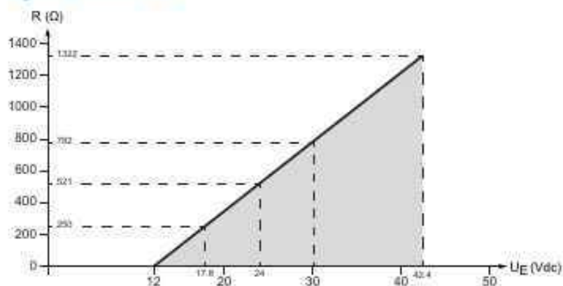
Figure 3: Load Limits
