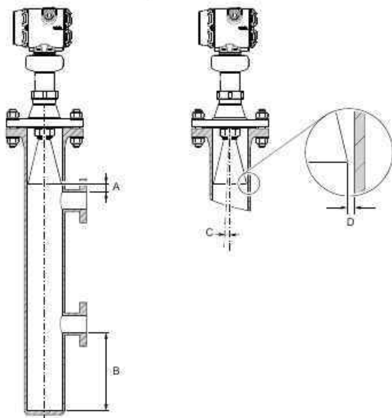
Figure 24: Chamber Requirements
