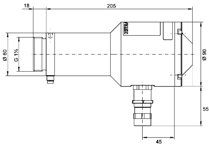
Fig. 6 Dimensional drawing compact flame scanner F200K Ex (for Ex zone 1, 21)
